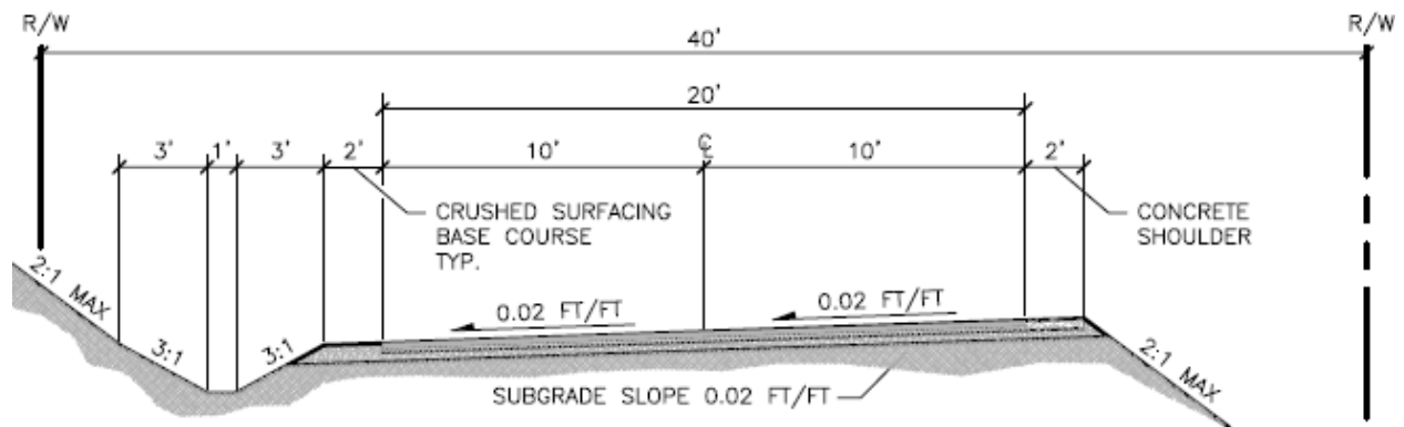
TYPE R-II MINOR RESIDENTIAL ROADWAY NOT TO SCALE
