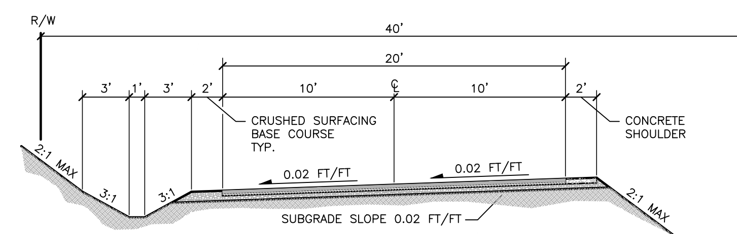
TYPE R-II (HERITAGE LANE) MINOR RESIDENTIAL ALT #2 ROADWAY NOT TO SCALE
