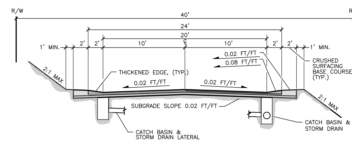
TYPE R-II (LEGACY TRAIL) MINOR RESIDENTIAL ROADWAY NOT TO SCALE
